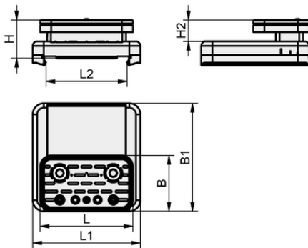
Design data VCBL-S4 125x75x50 TV
