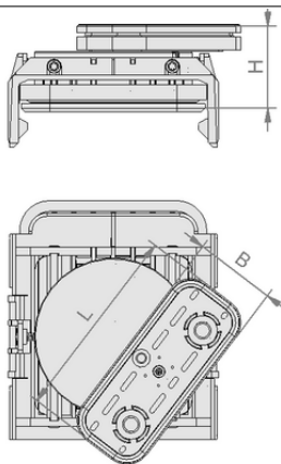
Design data VCBL-K1 125x75x125 D-360
