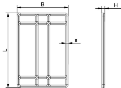
Design data VCDR 166x113x6.6 VCSP
