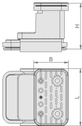
Design data VCBL-K2 120x50x125 Q
