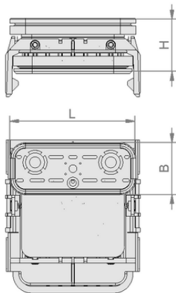
Design data VCBL-K1 120x50x85 Q
