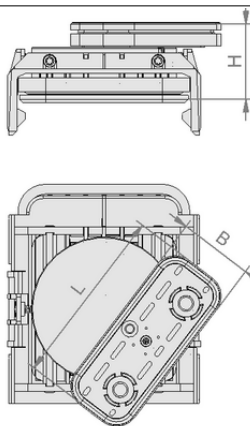
Design data VCBL-K1 125x75x85 D-360
