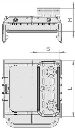
Design data VCBL-K1 125x75x85 L
