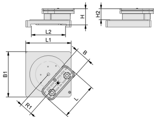
Design data VCBL-S4 120x50x50 D-360 TV
