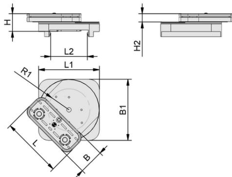
Design data VCBL-S1 120x50x32.7 D-360 TV
