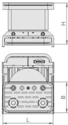
Design data VCBL-K2 125x75x100 D-360
