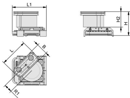
Design data VCBL-K2 120x50x100 D-360
