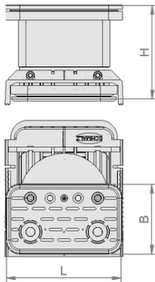
Design data VCBL-K2 120x50x50 D-360
