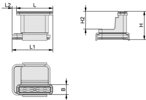
Design data VCBL-K2 130x30x100 L
