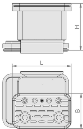
Design data VCBL-K2 125x75x50 L
