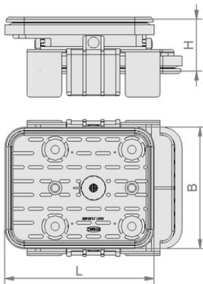
Design data VCBL-K1 140x115x50 TV
