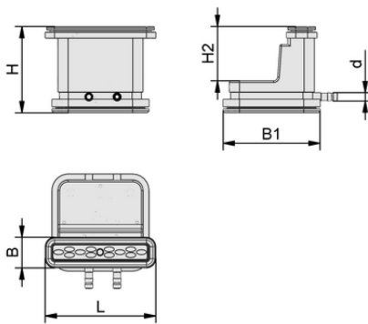
Design data VCBL-G-K2 130x30x100 ST
