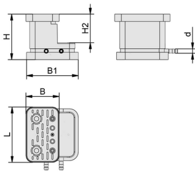
Design data VCBL-G-K2 125x75x100 ST
