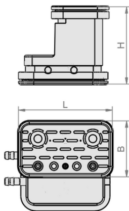
Design data VCBL-G-K2 120x50x100 ST
