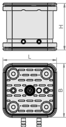
Design data VCBL-G-K2 120x120x100 ST+AS
