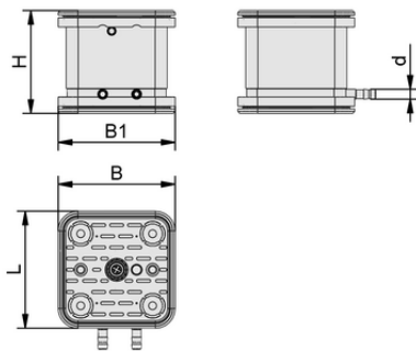
Design data VCBL-G-K2 120x120x100 ST
