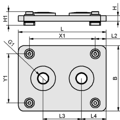
Design data FLAN-PL 160x120x10 FMHD
