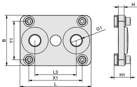
Design data FLAN-PL 120x85x10 ST FLGR
