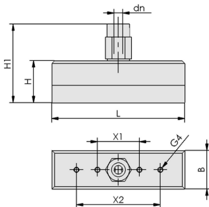
Design data FM-SW 38x22 N10
