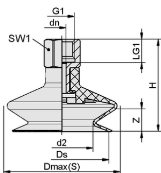
Design data FSGA 25 HT1-ESD-60 G1/8-IG
