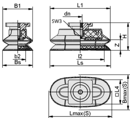
Design data SAOXB 110x55 ED-85 RA MOD
