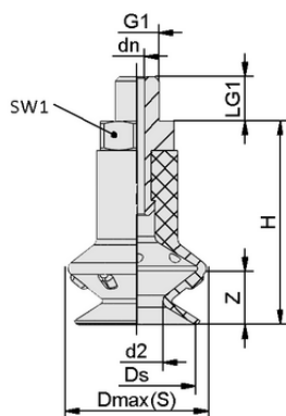
Design data FSGA 8 SI-40 M3-AG
