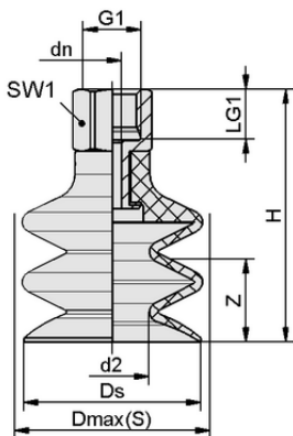
Design data FSG 25 SI-MD-55 G1/8-IG
