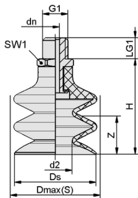
Design data FSG 12 SI-MD-55 G1/8-AG
