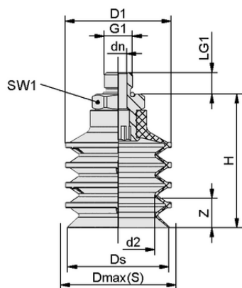
Design data FSGC 60 NBR-55 G1/4-AG
