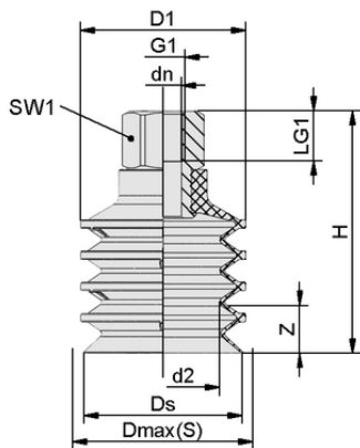
Design data FSGC 50 NBR-55 G1/4-IG
