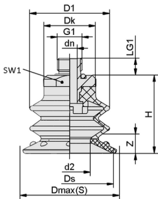
Design data SDC2 50 PU 30/60 G3/8-AG
