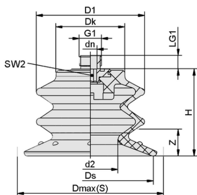
Design data SDC2 75 PU 30/60 G3/8-AG
