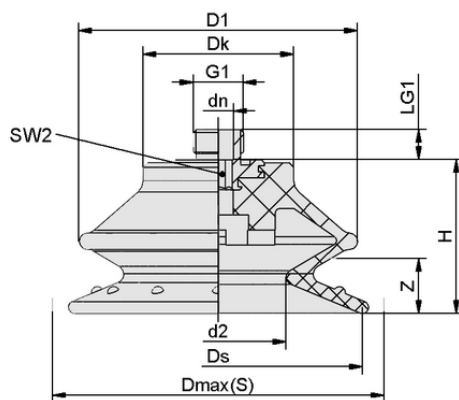
Design data SDC1 100 PU 30/60 G3/8-AG
