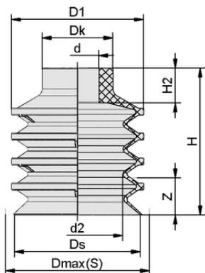
Design data FGC 50 NBR-55 SC080
