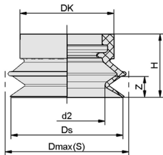
Design data BCG 40 SI-HD-65 SC095
