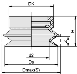
Design data BCG 30 SI-HD-65 SC085
