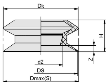
Design data FLSA 40 SI-MD-55
