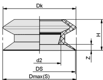
Design data FLSA 30 SI-MD-55
