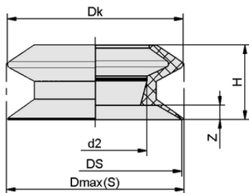
Design data FLSA 20 SI-MD-55
