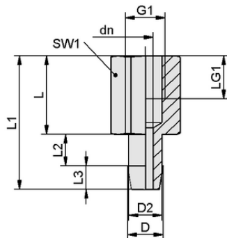
Design data SA-NIP N016 G1/8-IG DN310
