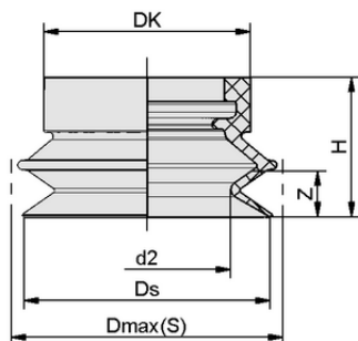
Design data BCG 50 NBR-ESD-55 SC095
