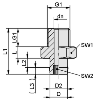
Design data SA-NIP N016 M5-AG DN250
