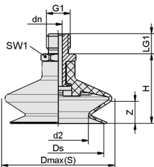
Design data FSGA 14 NBR-ESD-55 G1/8-AG
