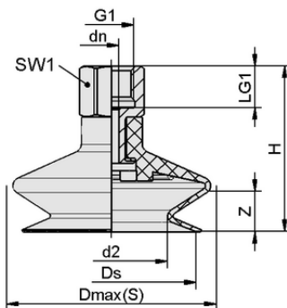
Design data FSGA 11 NBR-ESD-55 G1/8-IG
