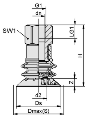
Design data SPB2f 20 SI-55 G1/8-IG
