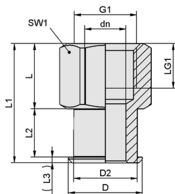
Design data SC 030 G1/8-IG
