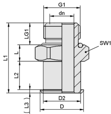
Design data SC 010 M3-AG
