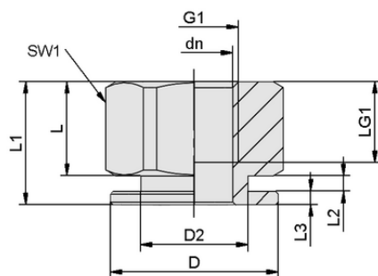
Design data SA-NIP N059 G1/4-IG
