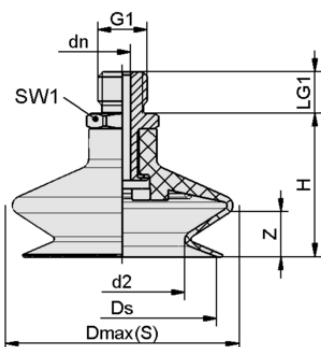
Design data FSGA 16 SI-MD-55 G1/8-AG
