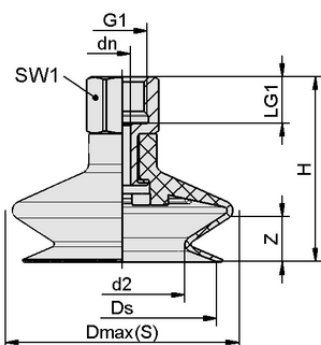
Design data FSGA 16 SI-HD-65 G1/8-IG
